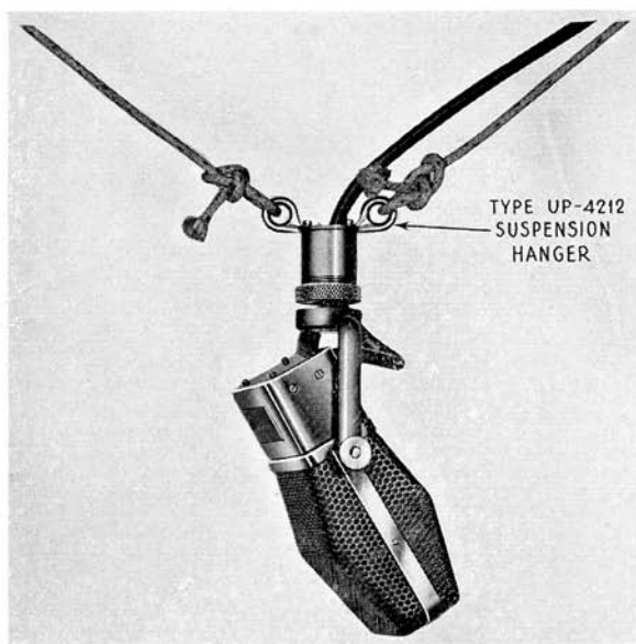
Figure 3—Microphone Suspended
