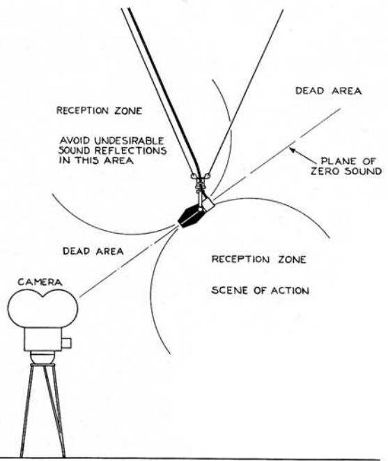
Figure 12—Camera Location for Sound Motion Picture Work
