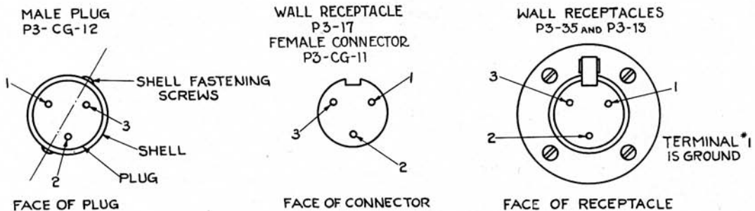
Figure 6—Plug and Receptacle Connections
