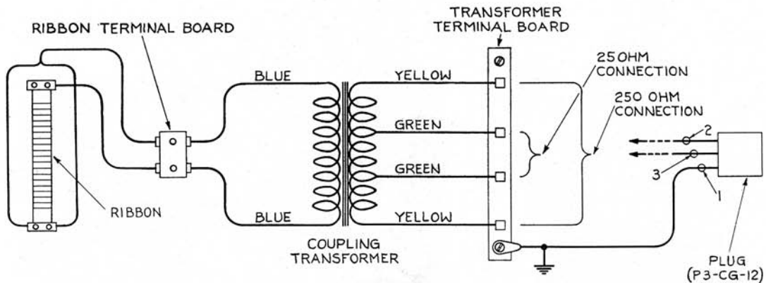
Figure 5—Schematic Wiring Diagram of Microphone and Cable
