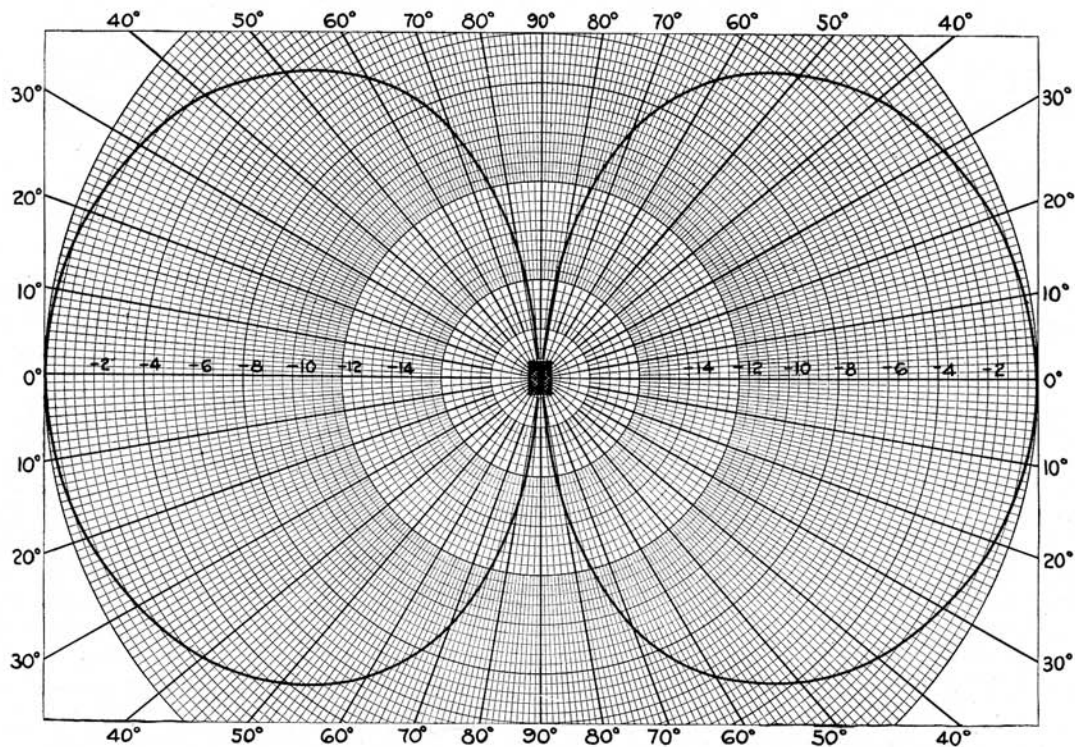
Figure 7—Directional Characteristics of Velocity Microphone
