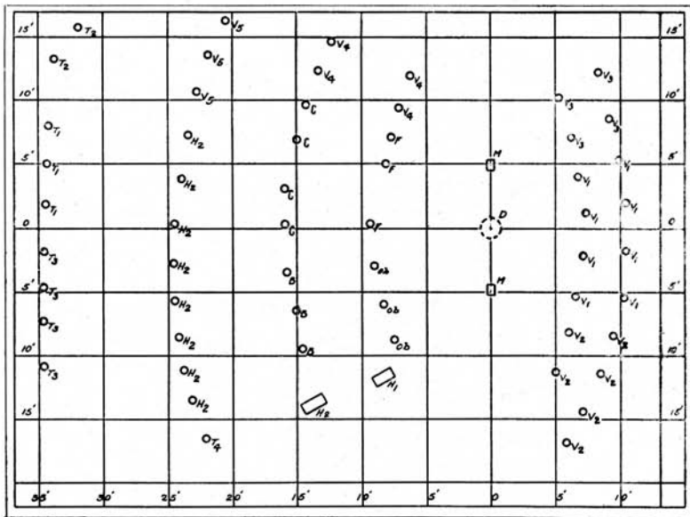
Figure 11—Microphone and Orchestra Arrangement for Symphony Orchestra
